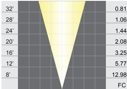
PAR36 LED: LED-5W-CPFL27K
