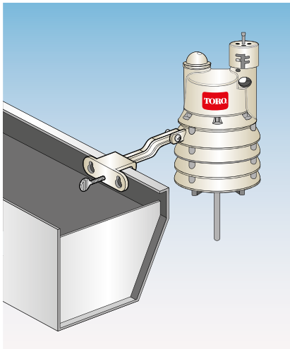
QuickClip™ Gutter Bracket
