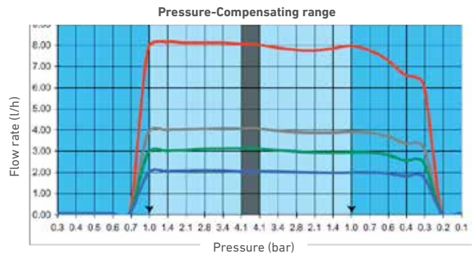
DRIPPER FLOW RATE VS. PRESSURE
