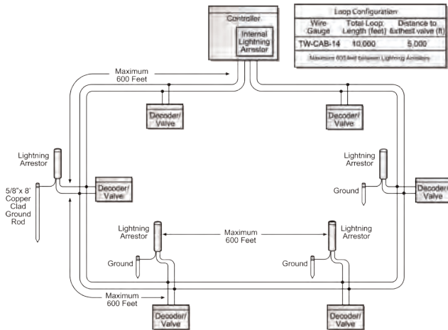
Loop Configuration
