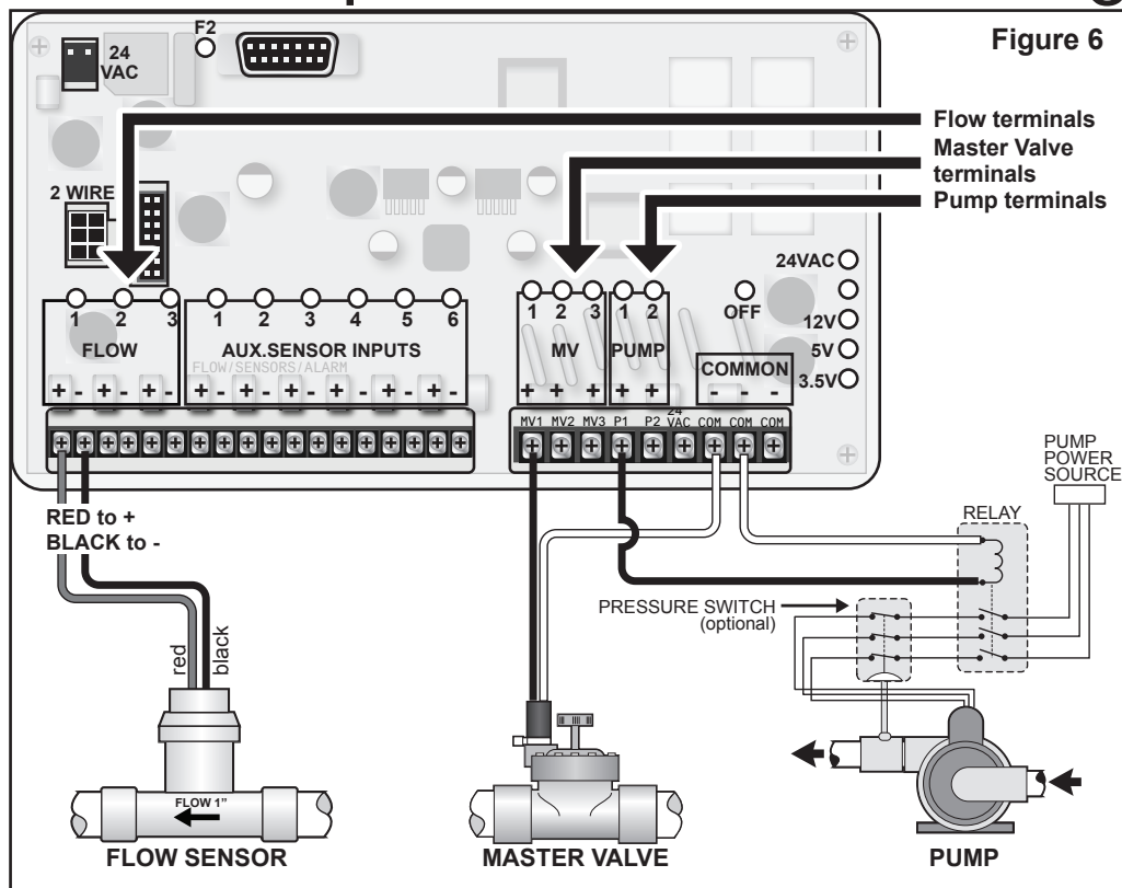
Master Valve, Pump, and Flow Sensor Wiring
