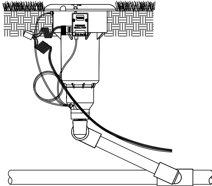
SECTION/ELEVATION NOT TO SCALE
