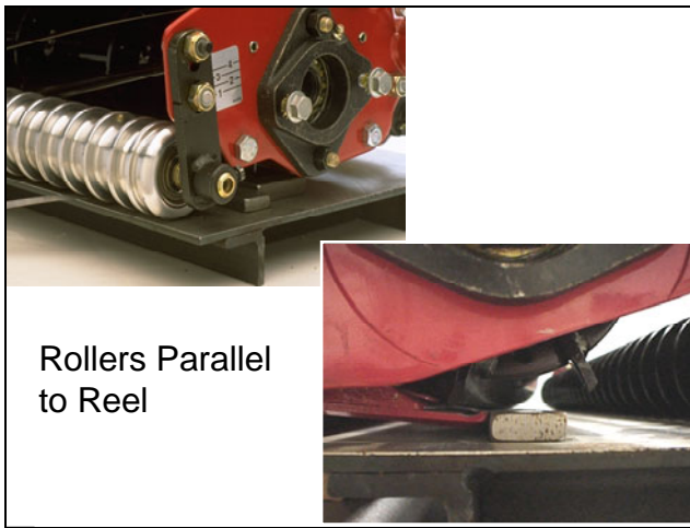
Height of Cut (H.O.C.)
