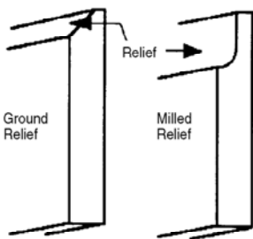
Milled Relief (Scalloped Blades)
