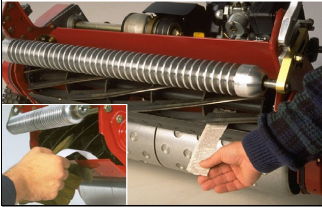
Parallel, Light Contact and Sharp
