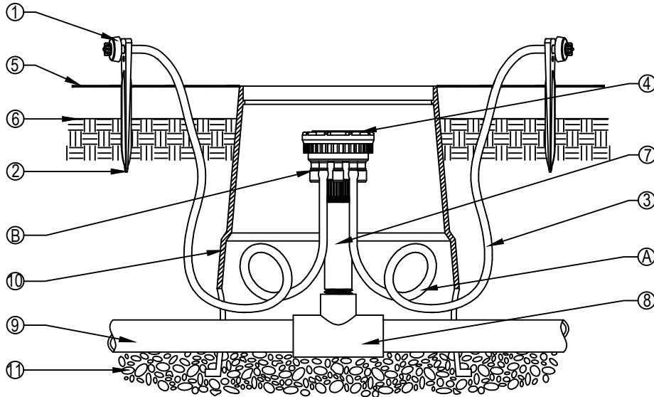
SECTION/ELEVATION
