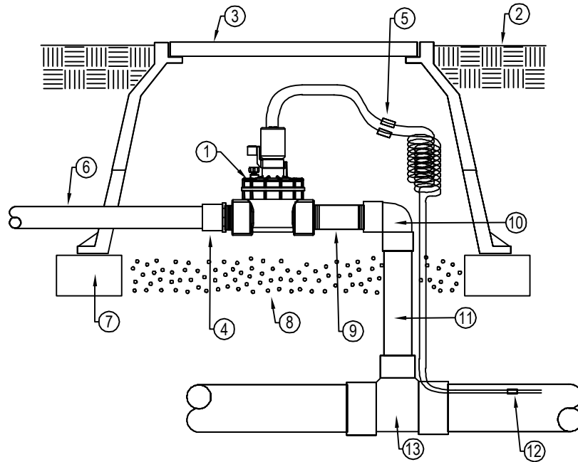
SECTION
