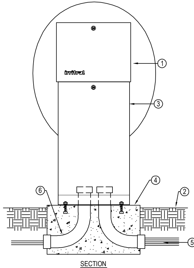
SECTION
